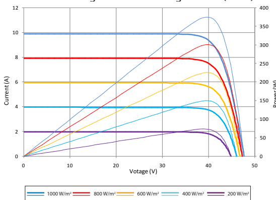
Current-Voltage & Power-Voltage Curve (375S)
